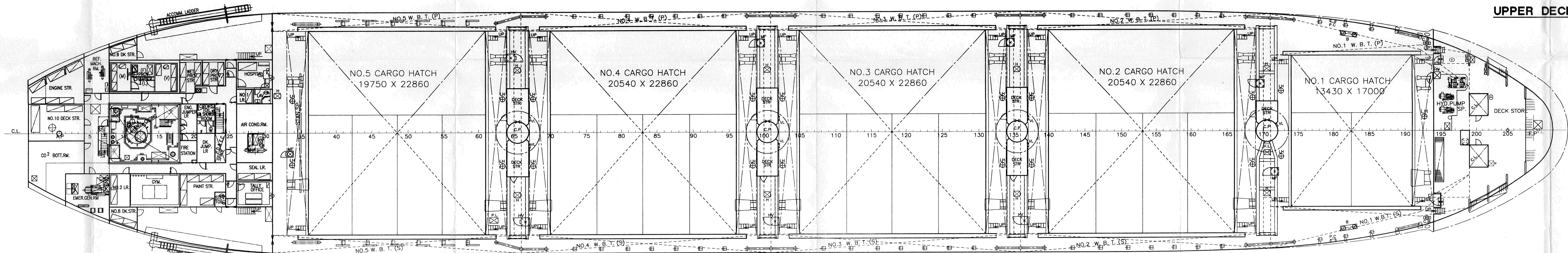
HOLD PLAN
