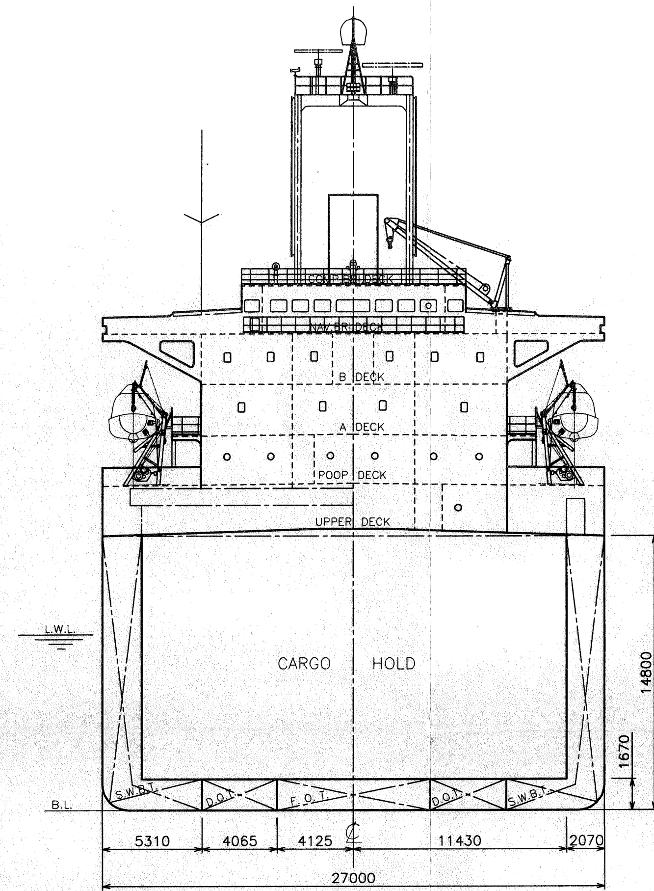
MIDSHIP & FRONT WALL SECTION
