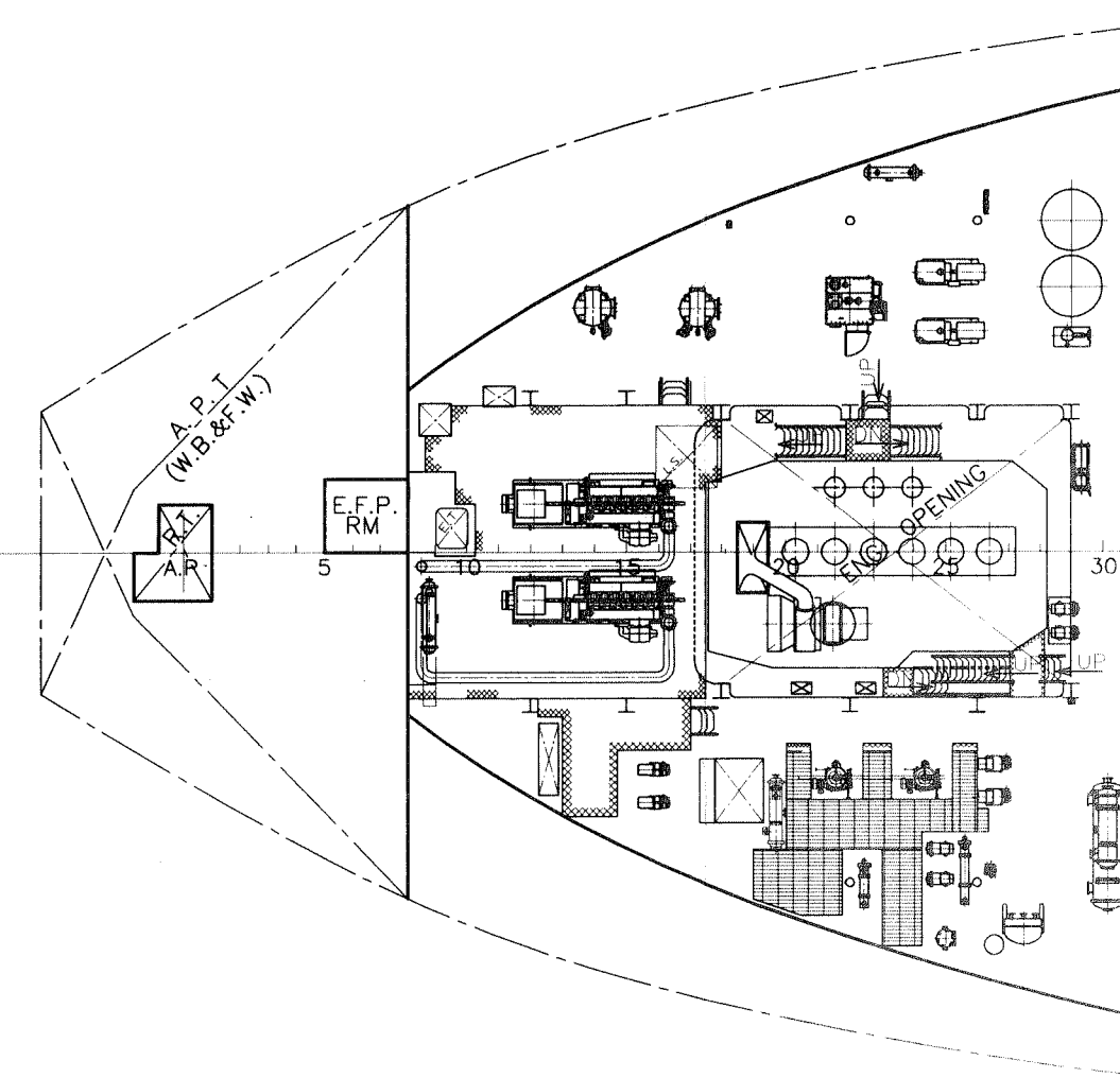
3RD DECK
