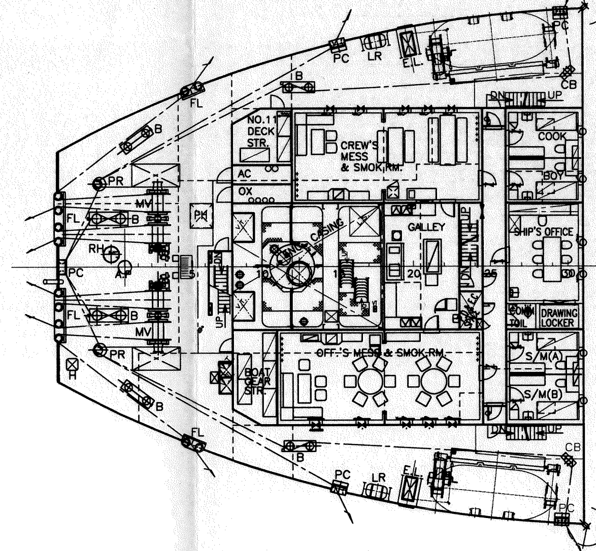
POOP DECK
