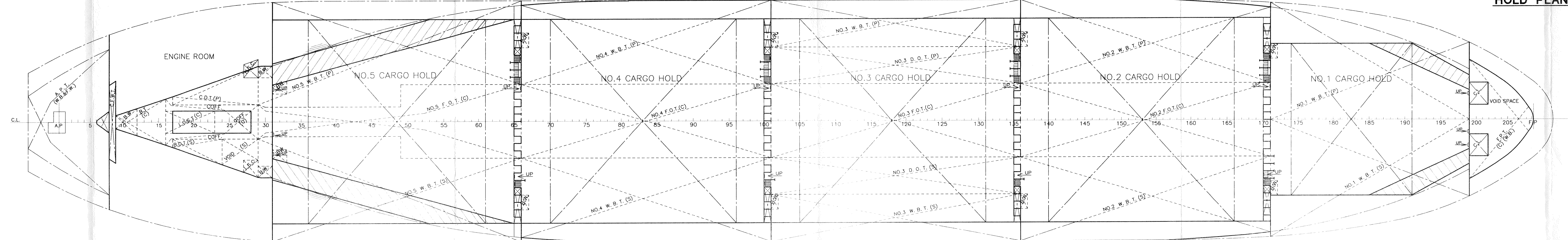
HOLD PLAN
