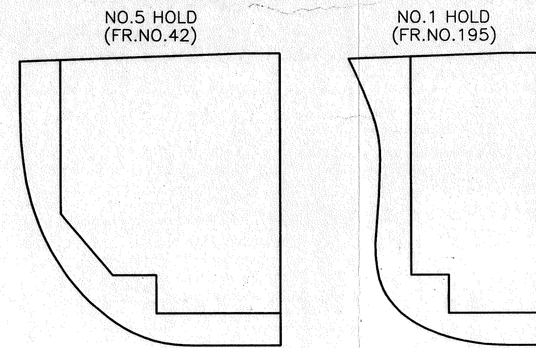
HOLD SECTION
