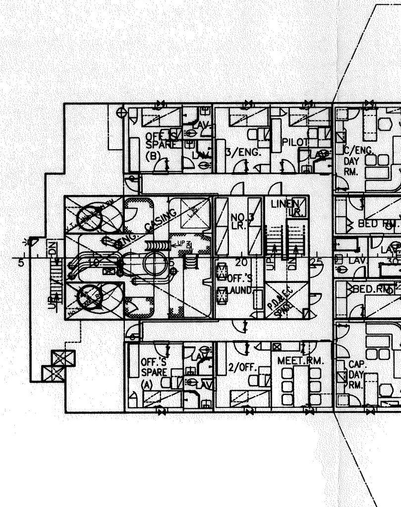
B-DECK
